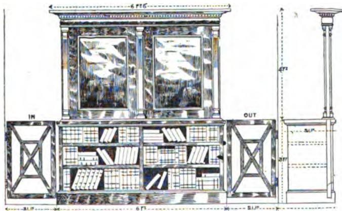
FIG. 23.—Elevation and Section of Barrier for an Open-Access Reference Library (Section 159).
